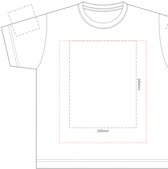
KIDS' SIZE 8 FRONT Print area can be rotated to best suit. Branding area can be moved anywhere within the red line.
