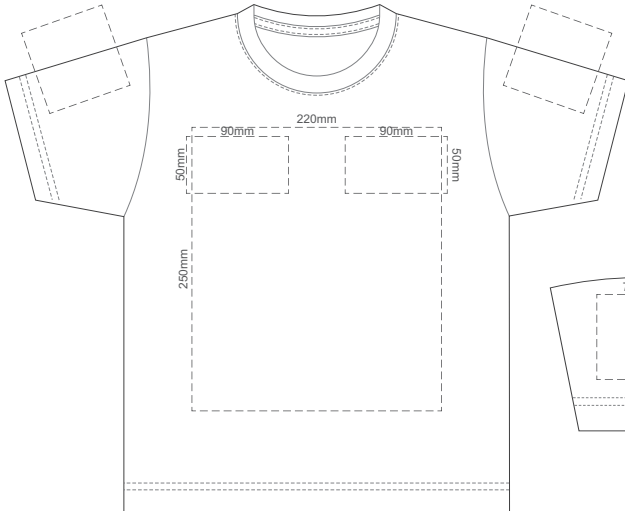
FRONT KID'S SIZE 4
